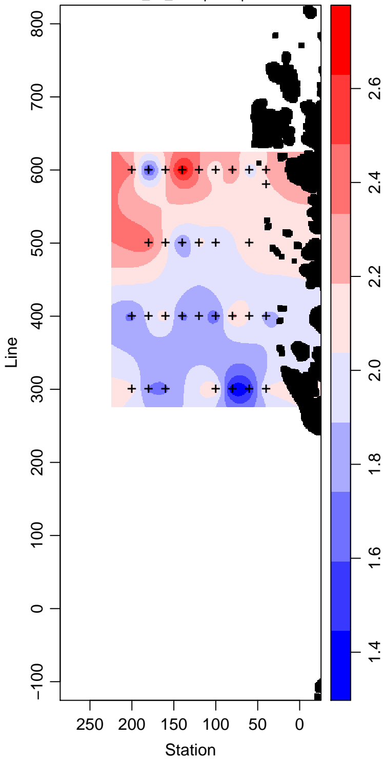
PD94-01_85_Phosphate \mu\text{ mol L}^{-1}
