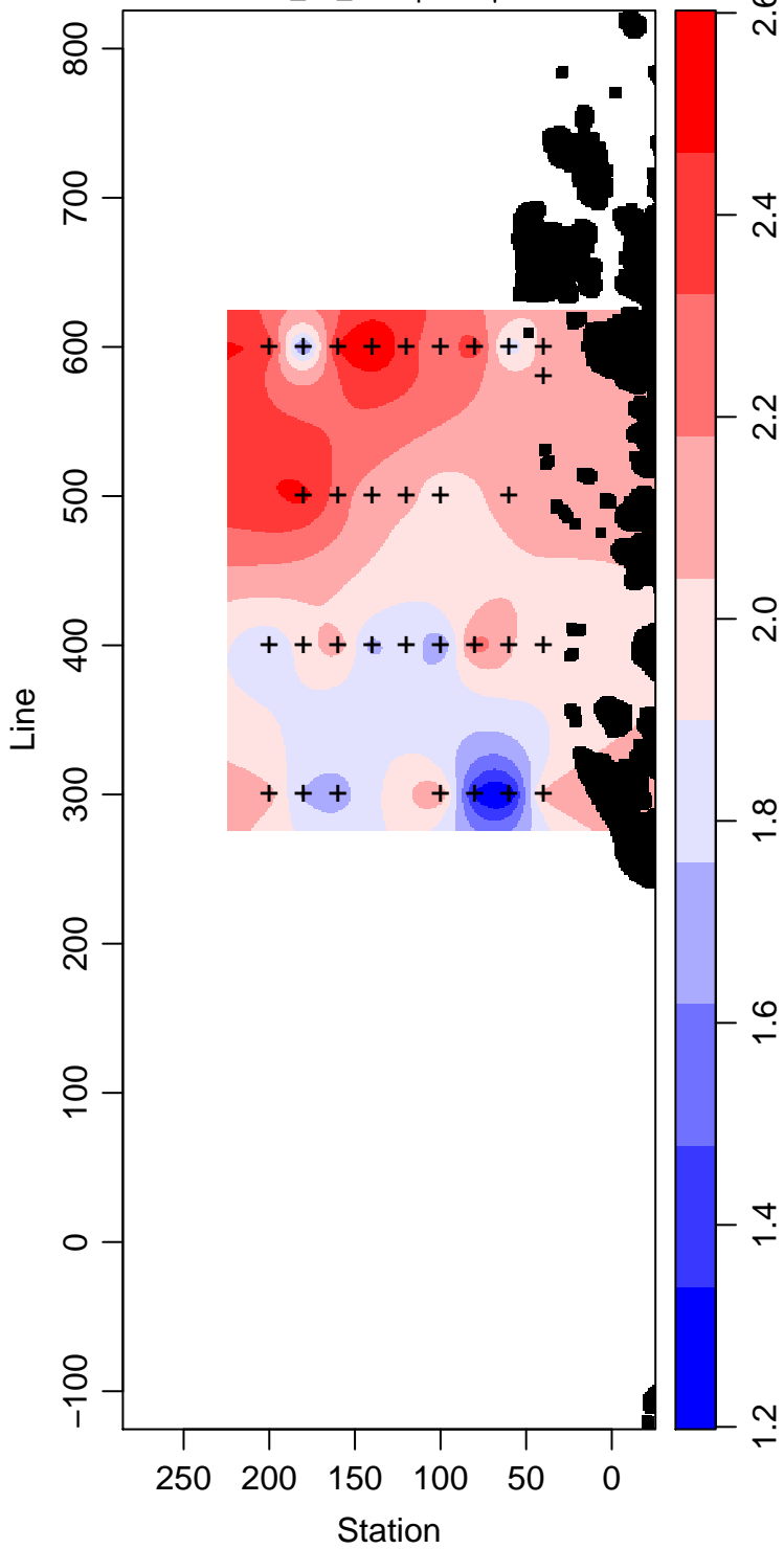
PD94-01_90_Phosphate \mu\text{ mol L}^{-1}
