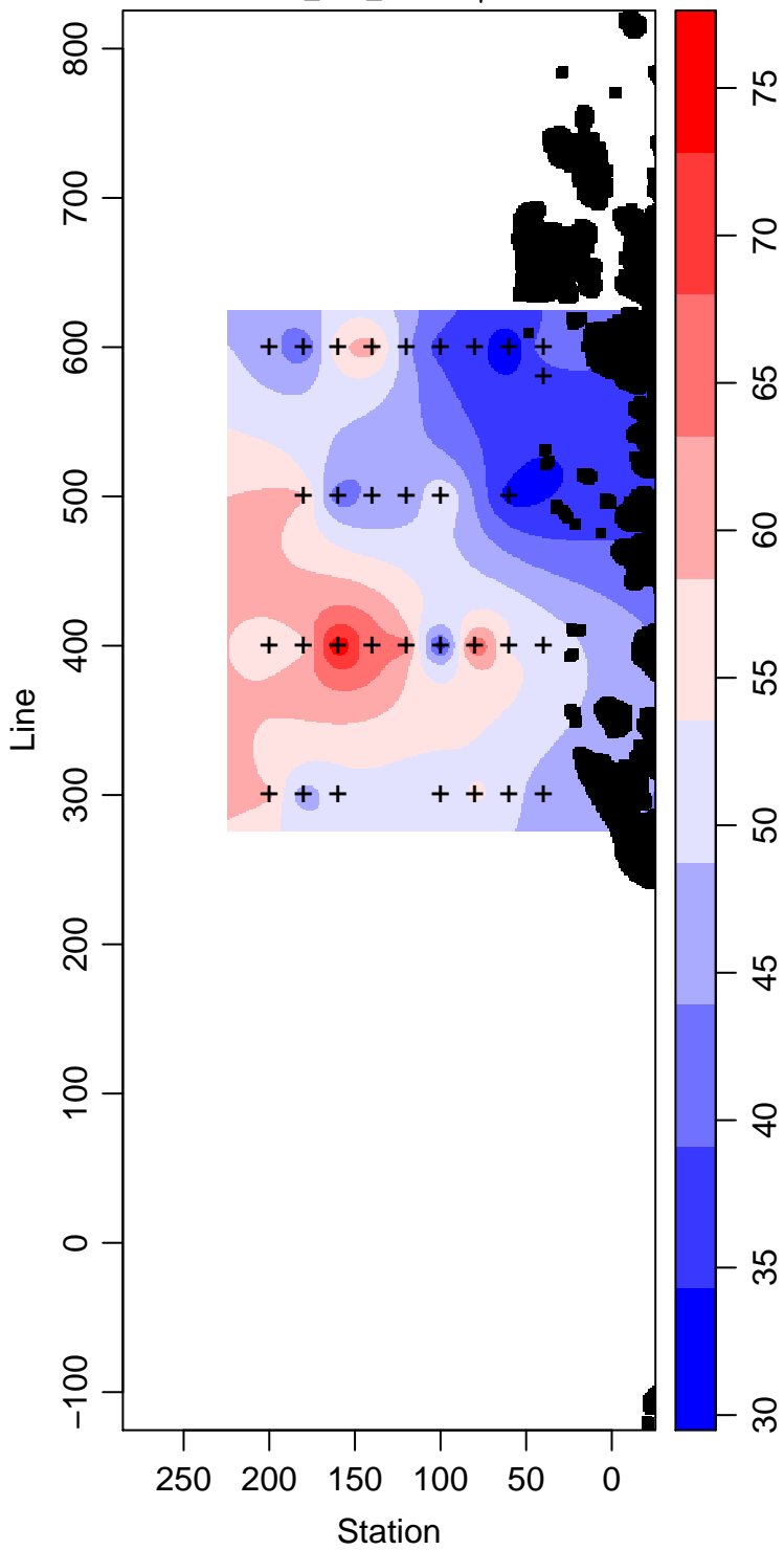
PD94-01_100_Silicate \mu\text{ mol L}^{-1}
