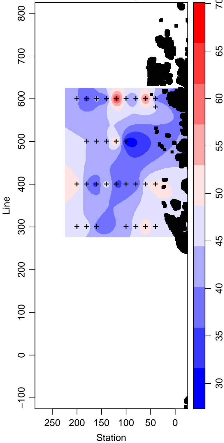
PD94-01_10_Silicate \mu\text{ mol L}^{-1}
