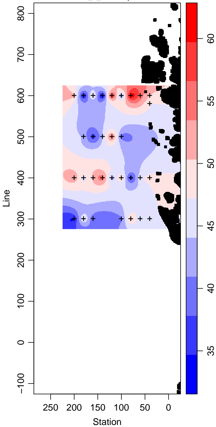
PD94-01_1_Silicate \mu\text{ mol L}^{-1}
