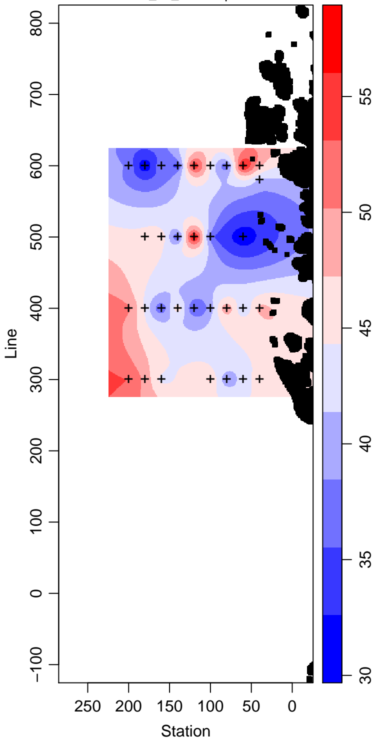
PD94-01_25_Silicate \mu\text{ mol L}^{-1}
