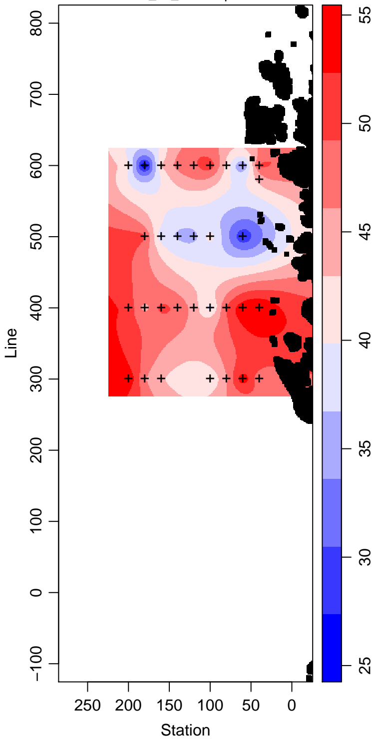
PD94-01_45_Silicate \mu\text{ mol L}^{-1}
