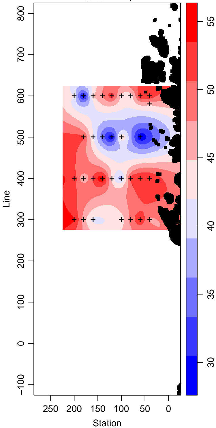
PD94-01_50_Silicate \mu\text{ mol L}^{-1}
