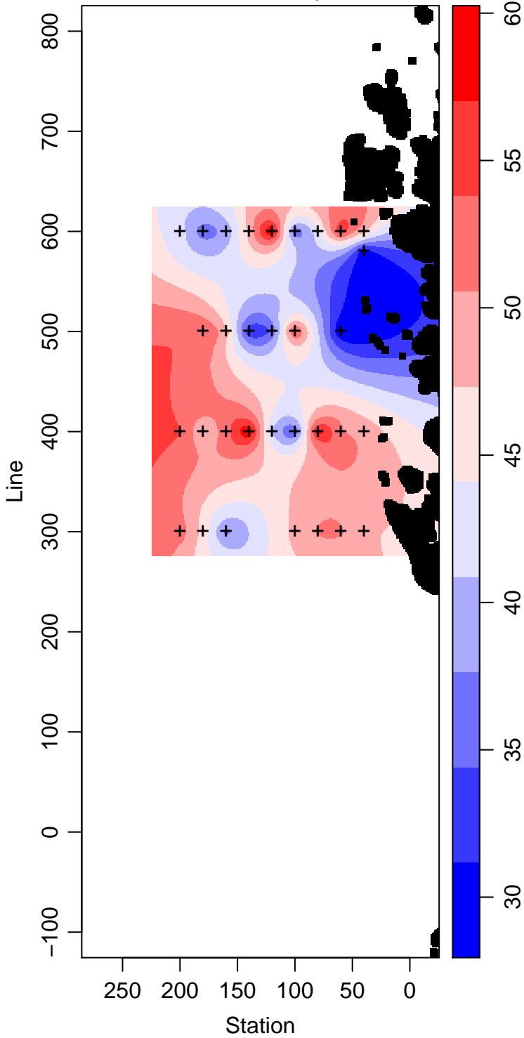
PD94-01_60_Silicate \mu\text{ mol L}^{-1}
