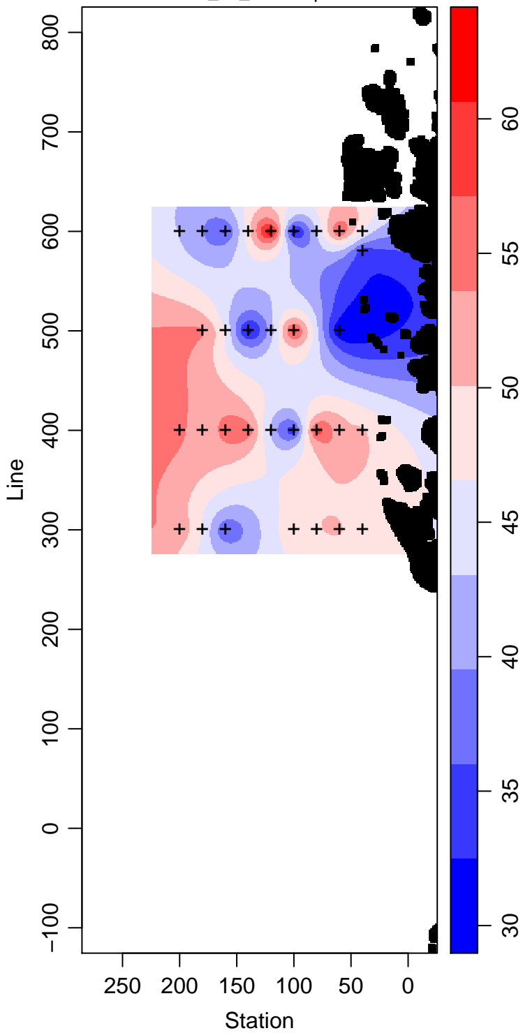
PD94-01_65_Silicate \mu\text{ mol L}^{-1}
