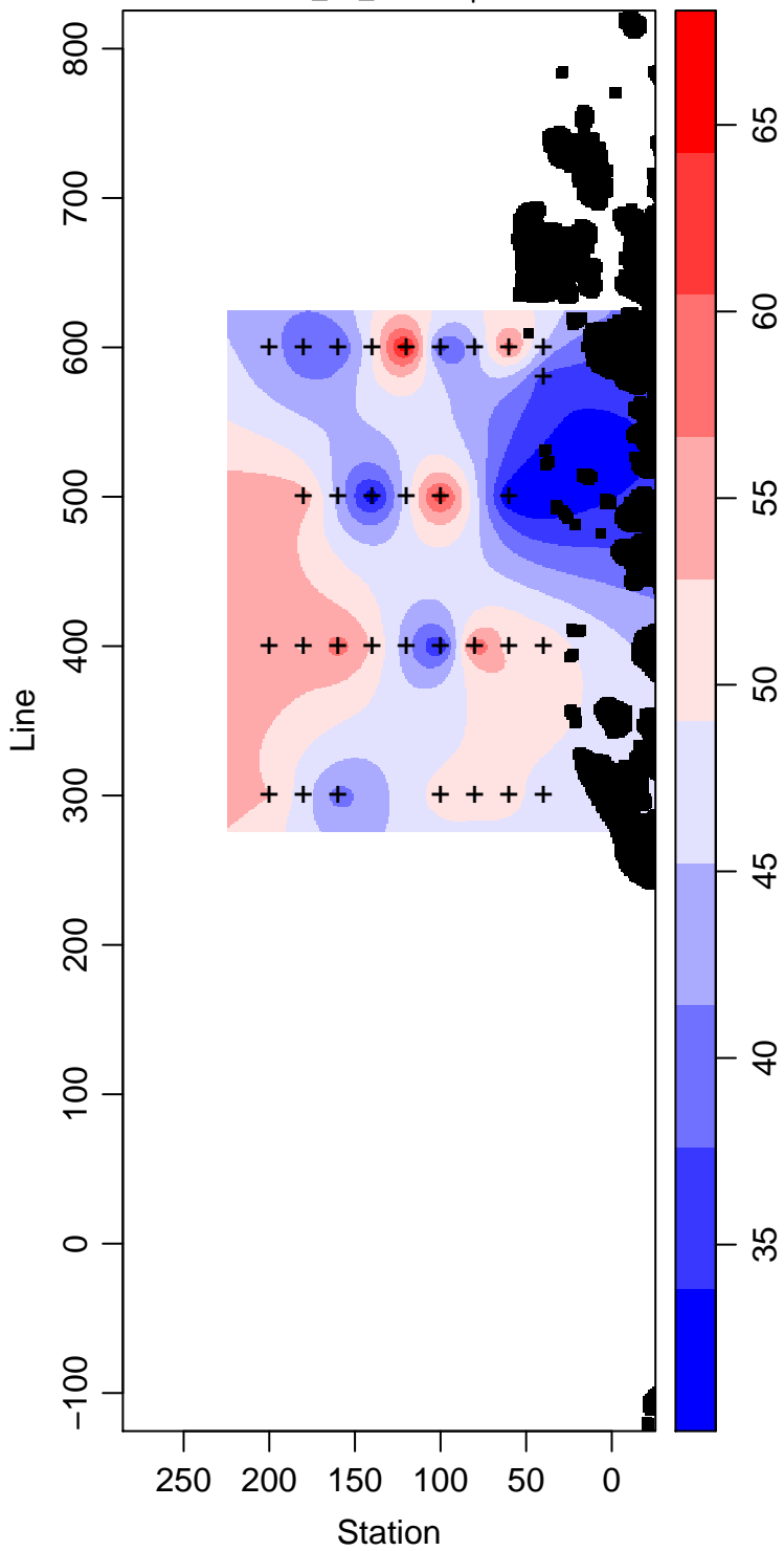
PD94-01_70_Silicate \mu\text{ mol L}^{-1}
