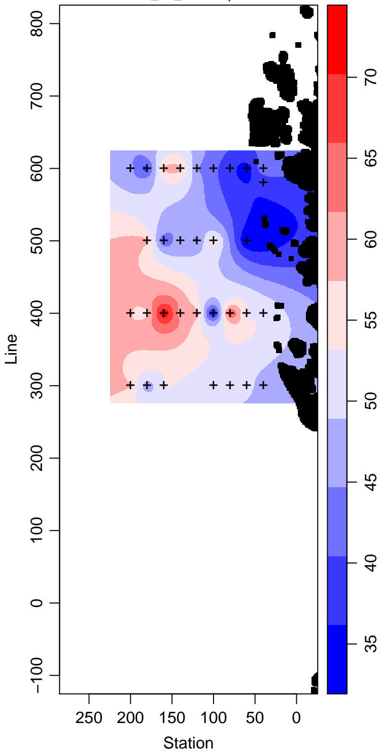
PD94-01_95_Silicate \mu\text{ mol L}^{-1}
