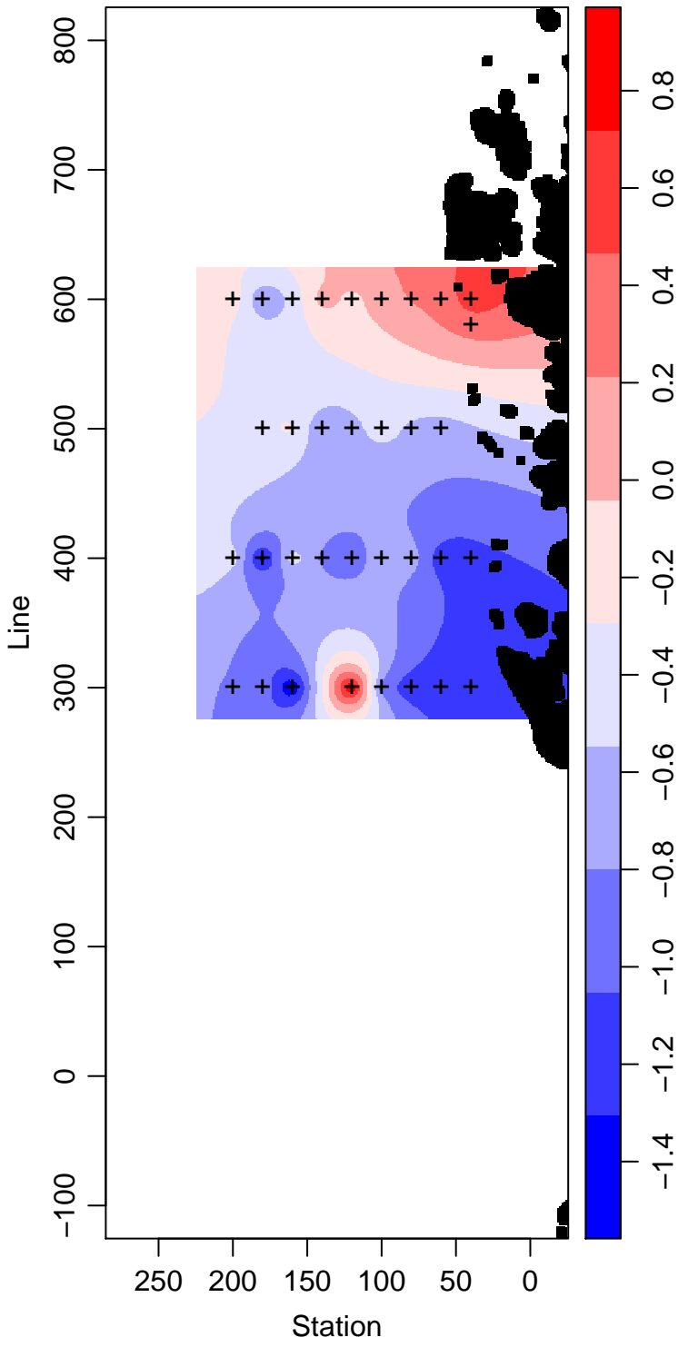
PD94-01_100_Temperature ° Celsius
