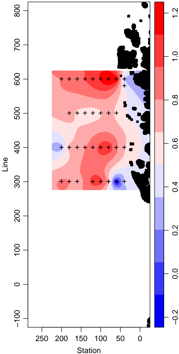
PD94-01_10_Temperature ° Celsius
