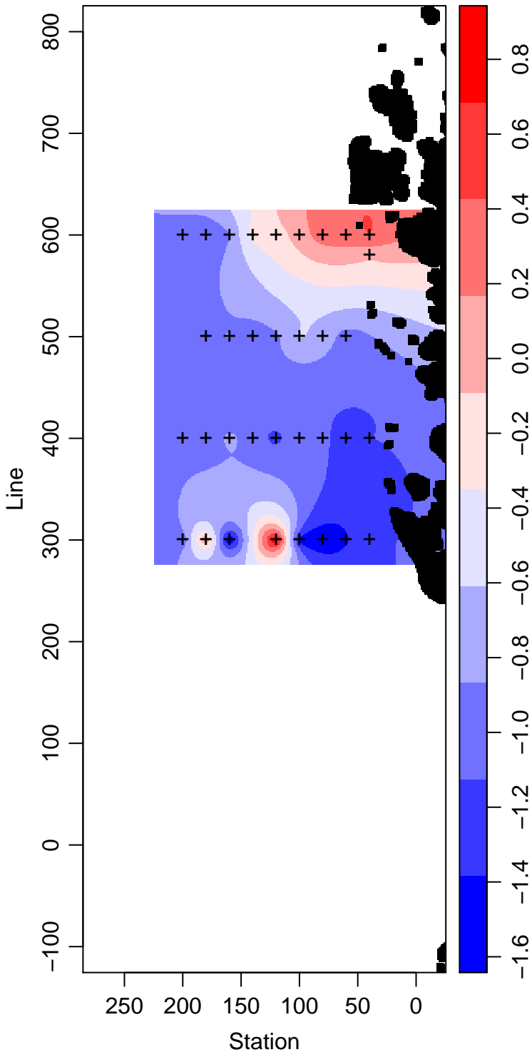
PD94-01_80_Temperature ° Celsius
