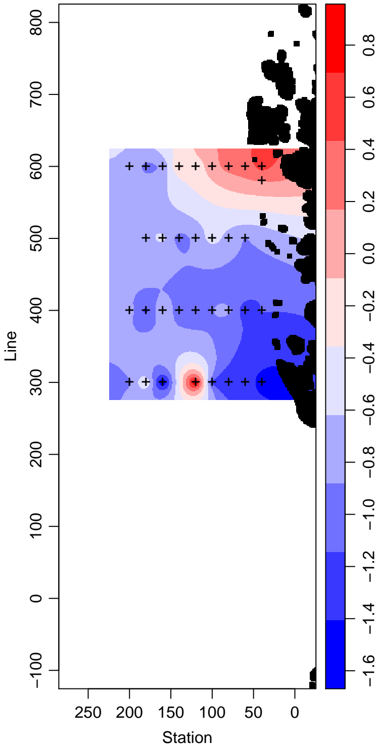
PD94-01_90_Temperature ° Celsius
