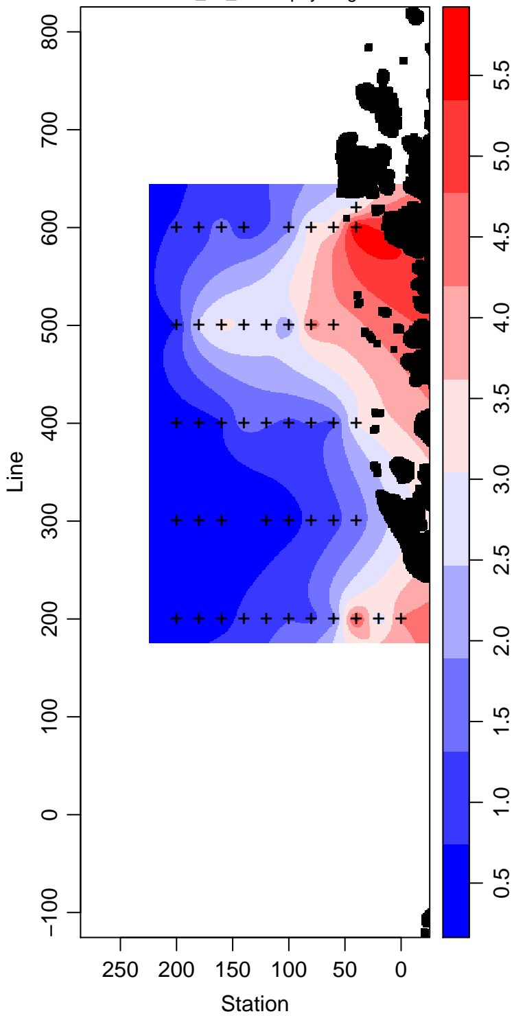
PD95-01_20_Chlorophyll mg m -3
