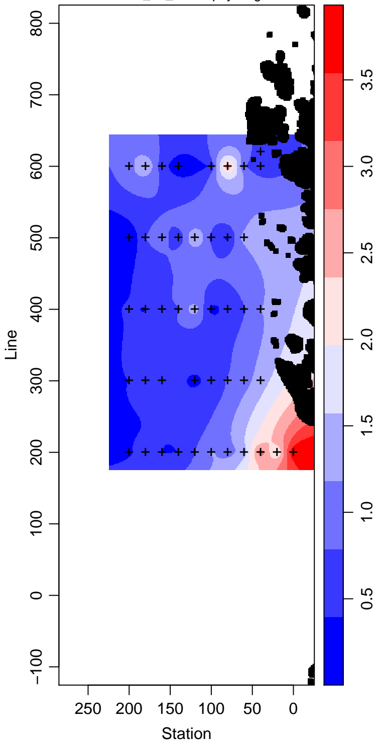
PD95-01_55_Chlorophyll mg m -3
