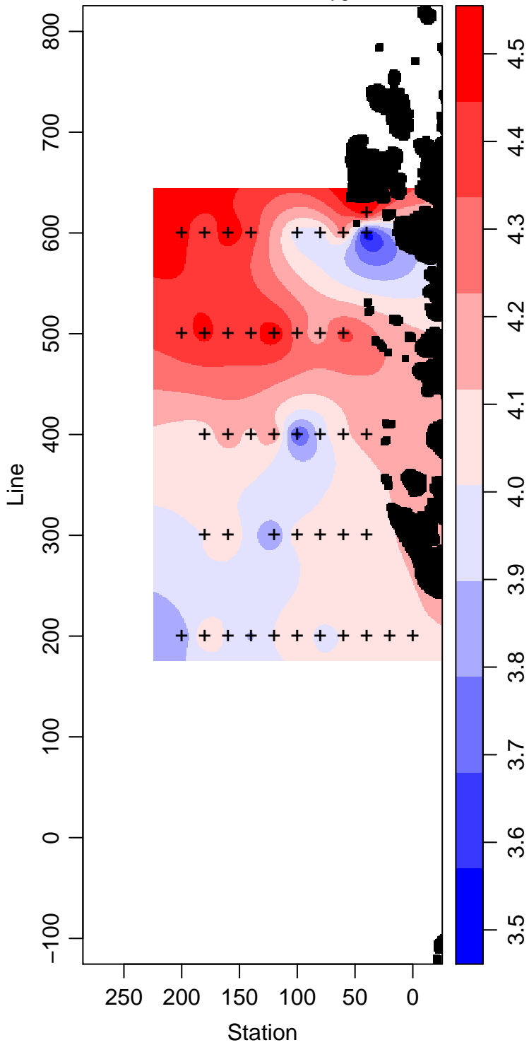
PD95-01_40_Dissolved.Oxygen ml L -1
