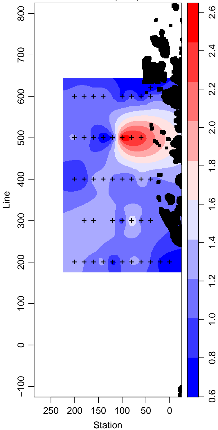
PD95-01_10_Phosphate \mu\text{ mol L}^{-1}
