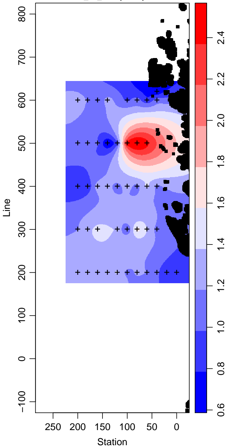
PD95-01_20_Phosphate \mu\text{ mol L}^{-1}
