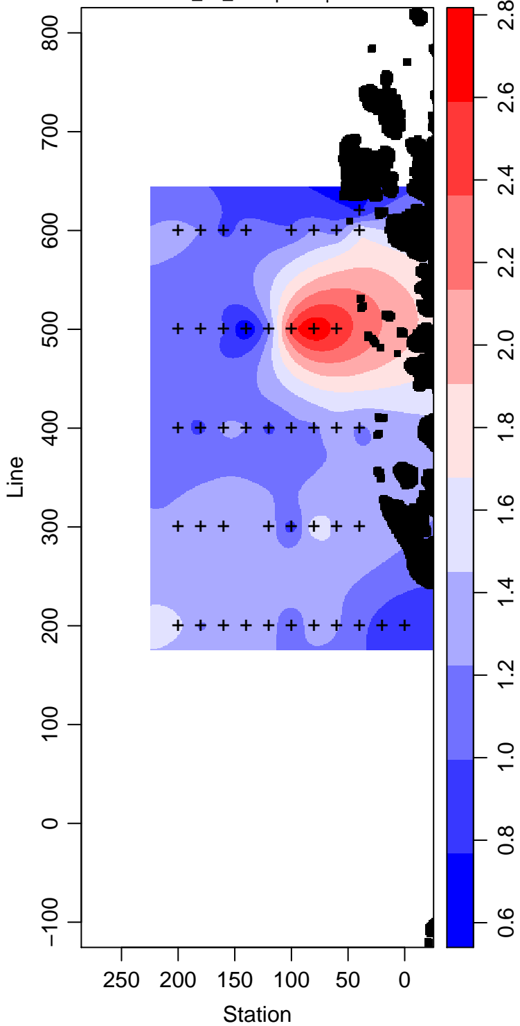
PD95-01_35_Phosphate \mu\text{ mol L}^{-1}
