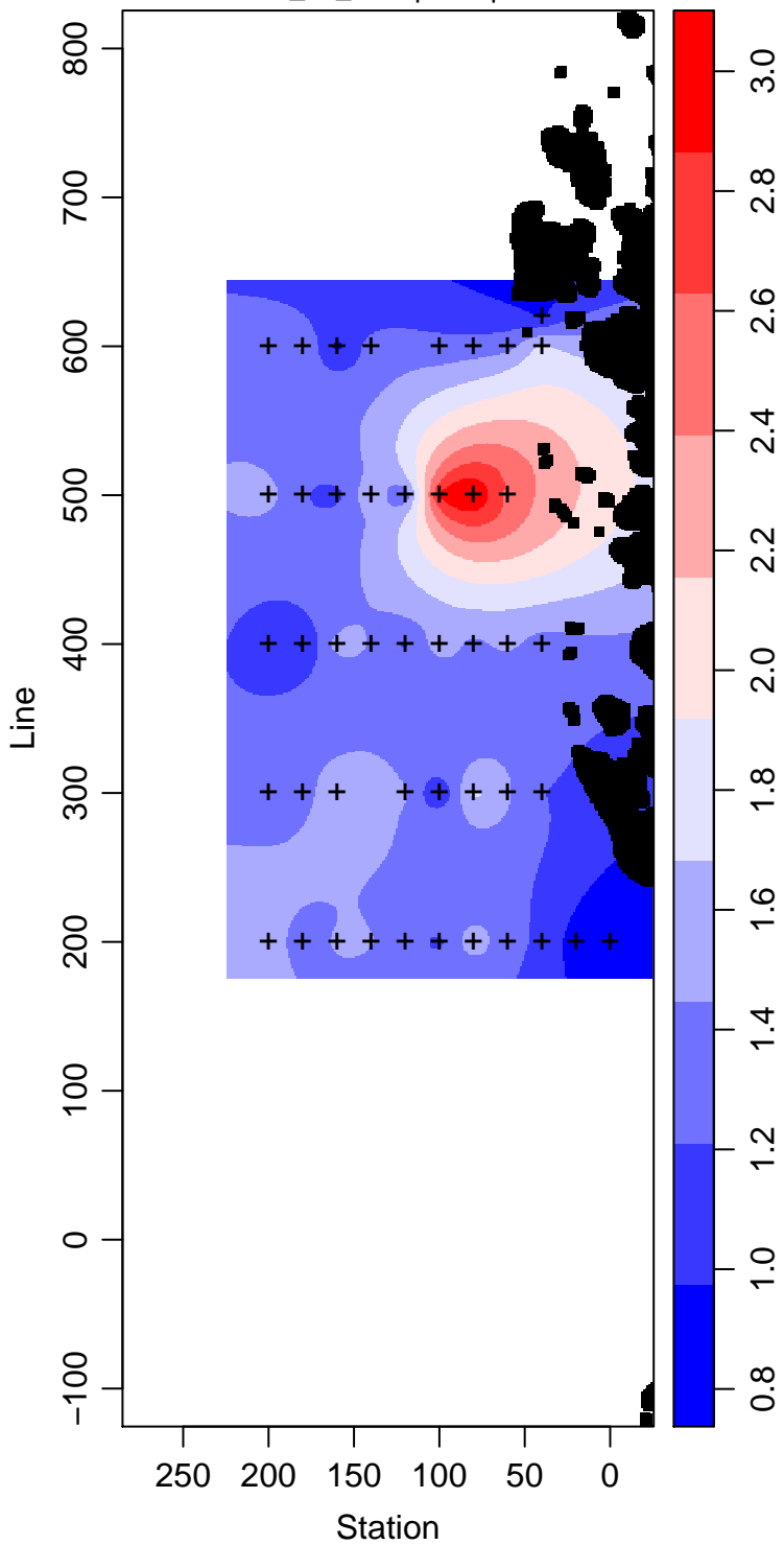
PD95-01_50_Phosphate \mu\text{ mol L}^{-1}
