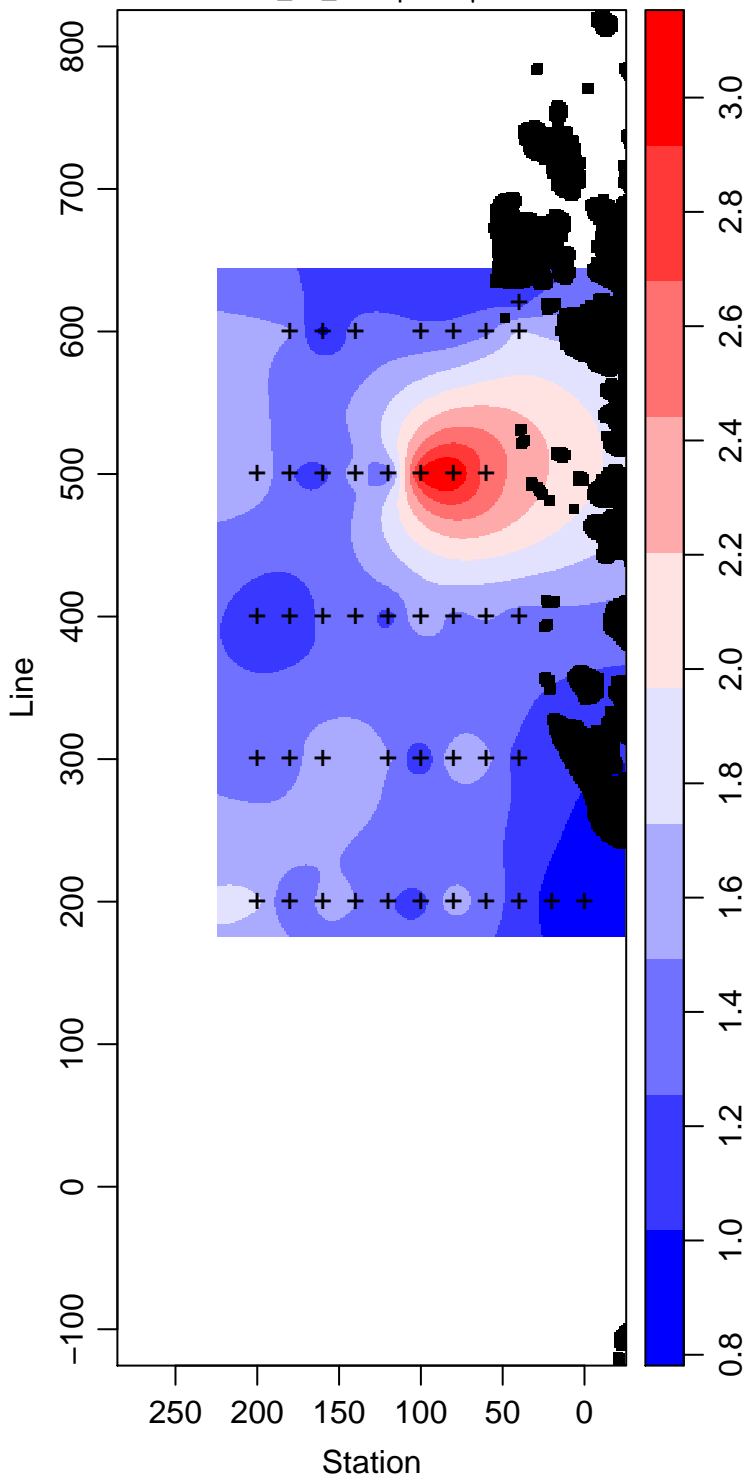
PD95-01_55_Phosphate \mu\text{ mol L}^{-1}
