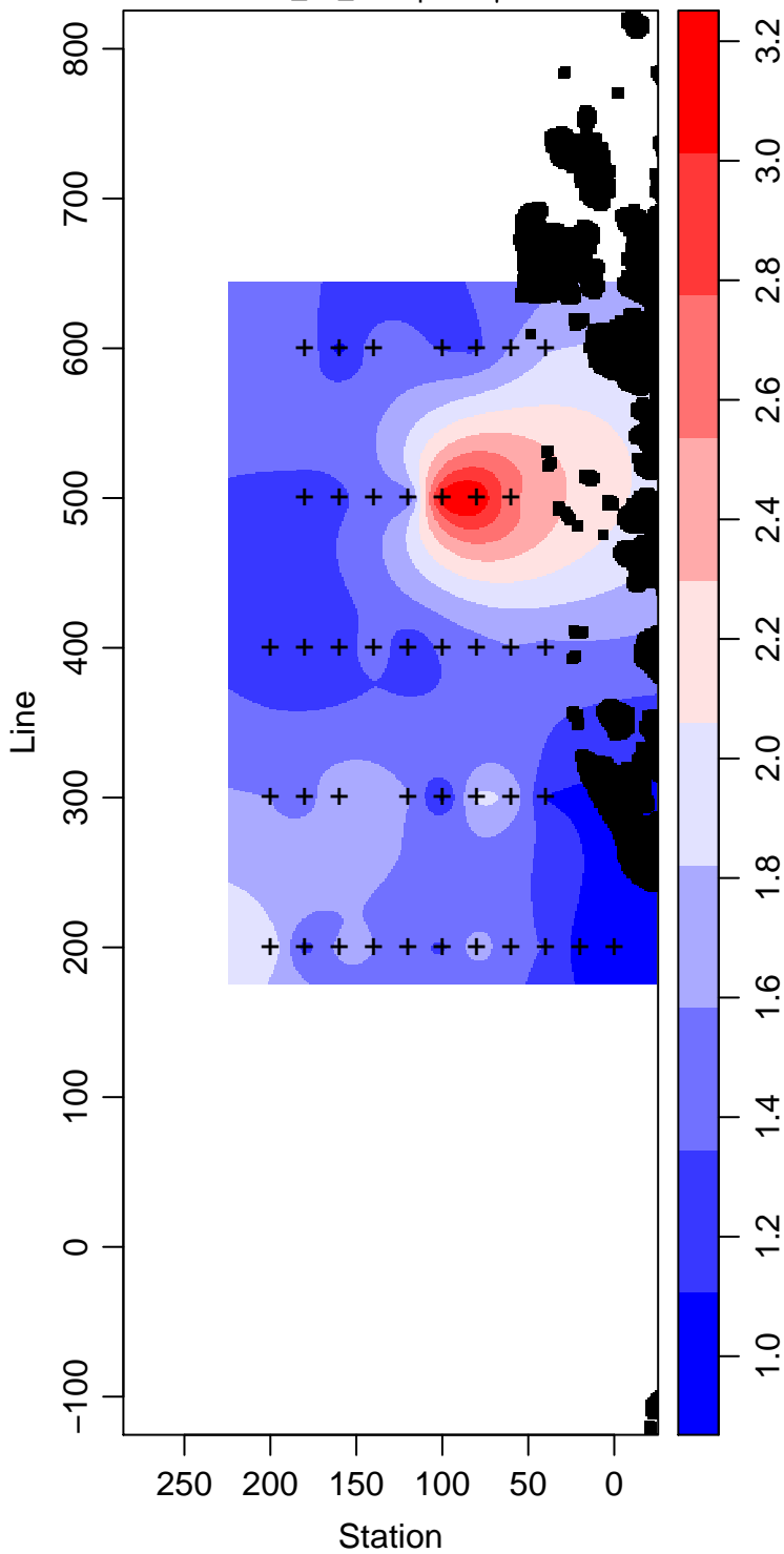
PD95-01_65_Phosphate \mu\text{ mol L}^{-1}
