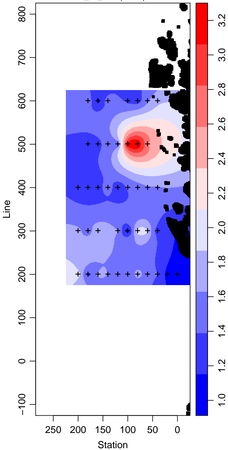
PD95-01_70_Phosphate \mu\text{ mol L}^{-1}
