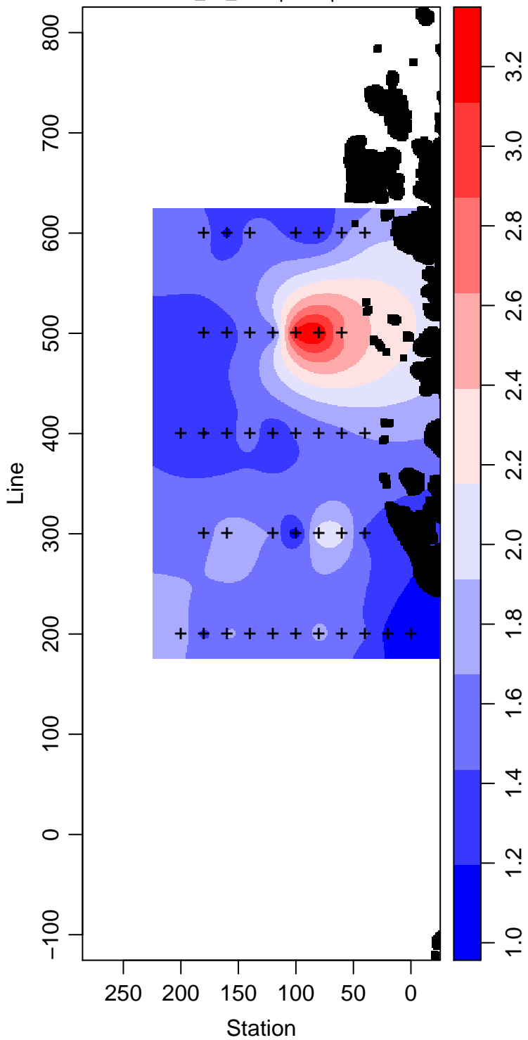
PD95-01_75_Phosphate \mu\text{ mol L}^{-1}
