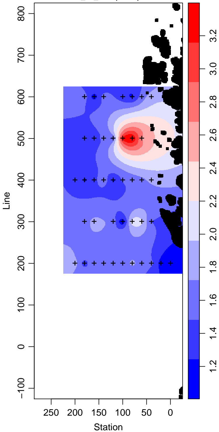
PD95-01_80_Phosphate \mu\text{ mol L}^{-1}
