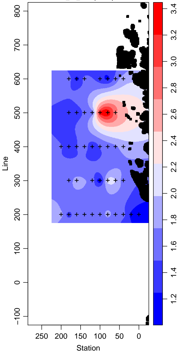
PD95-01_85_Phosphate \mu\text{ mol L}^{-1}
