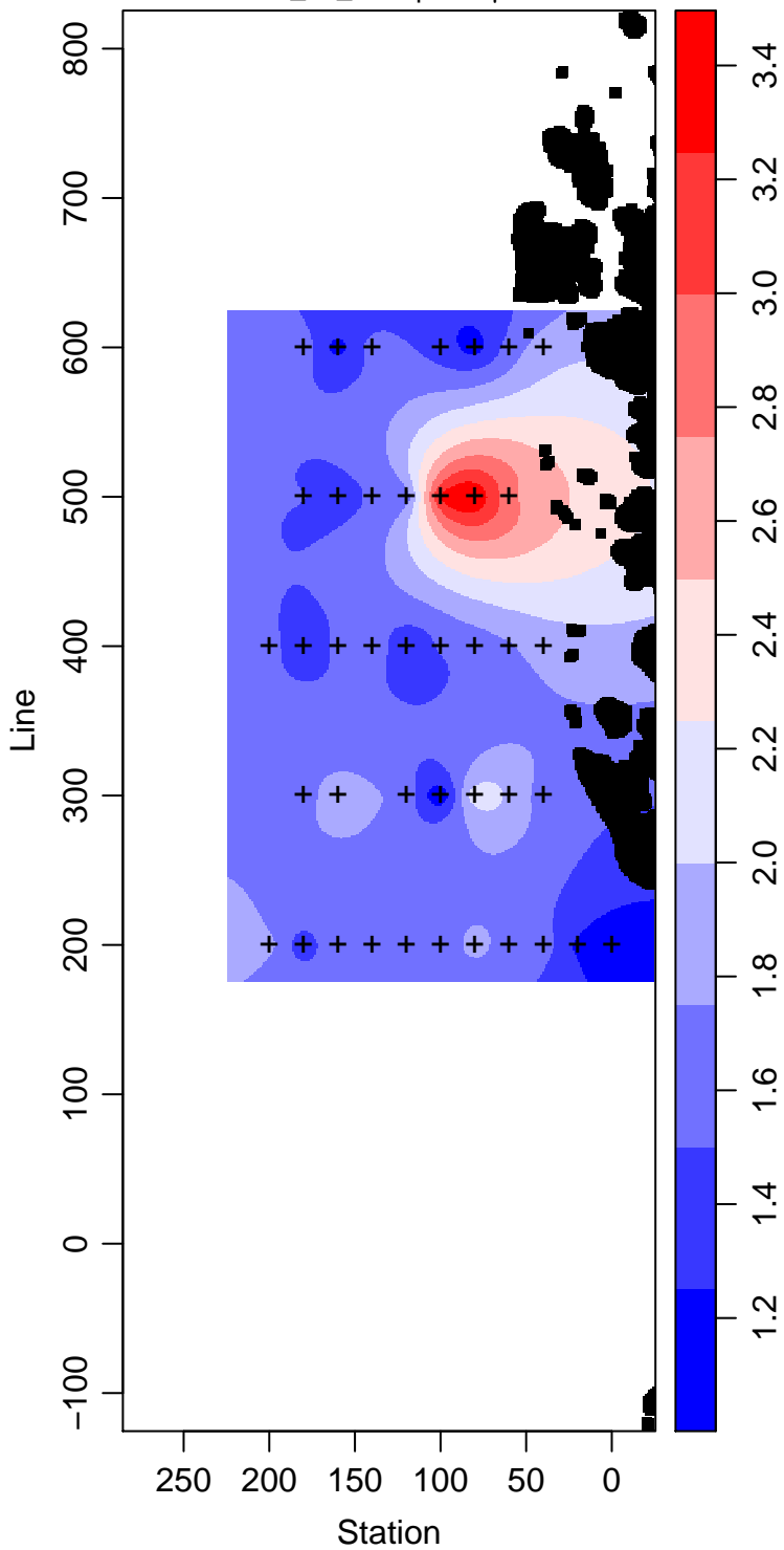
PD95-01_90_Phosphate \mu\text{ mol L}^{-1}
