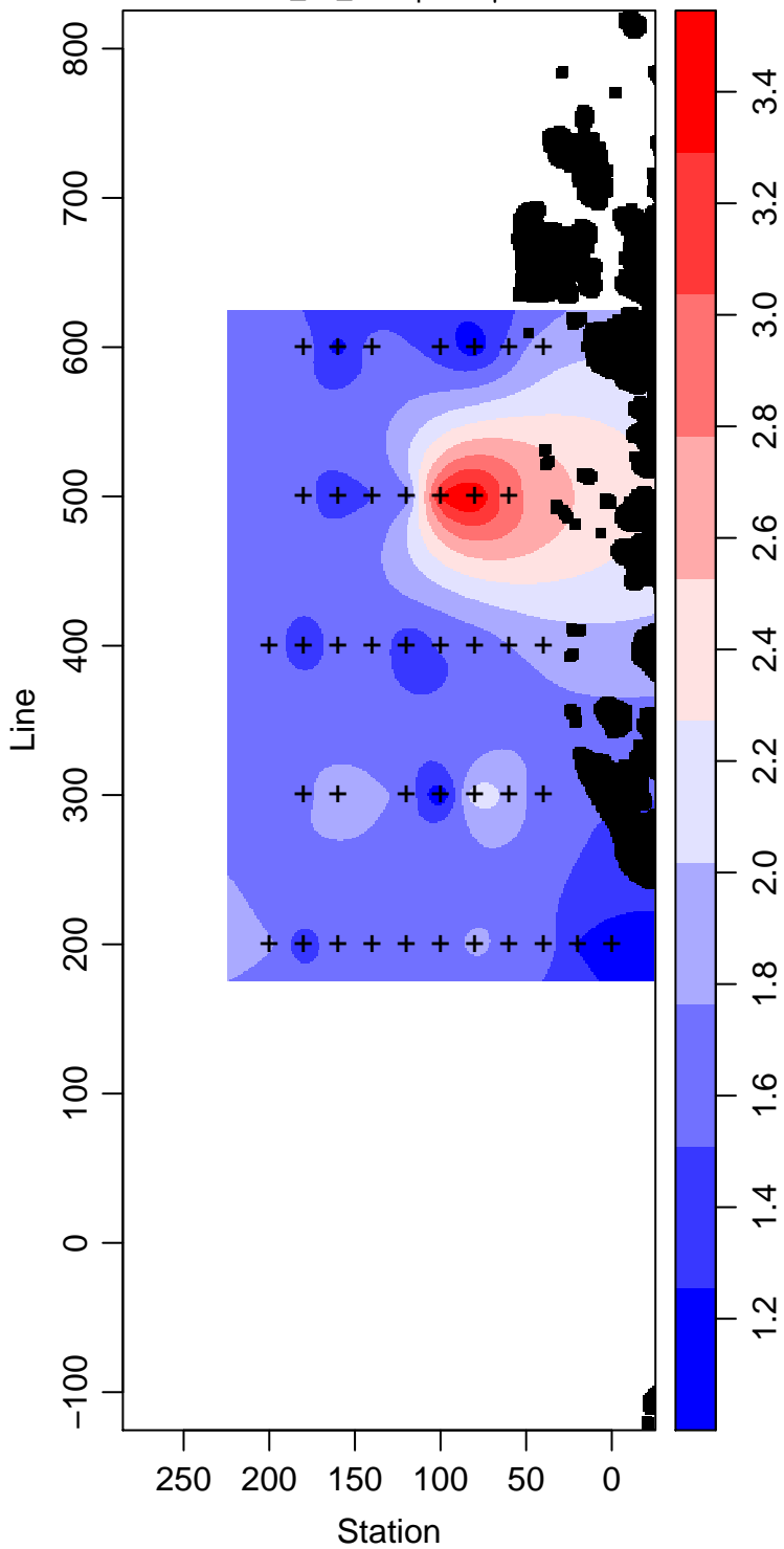
PD95-01_95_Phosphate \mu\text{ mol L}^{-1}
