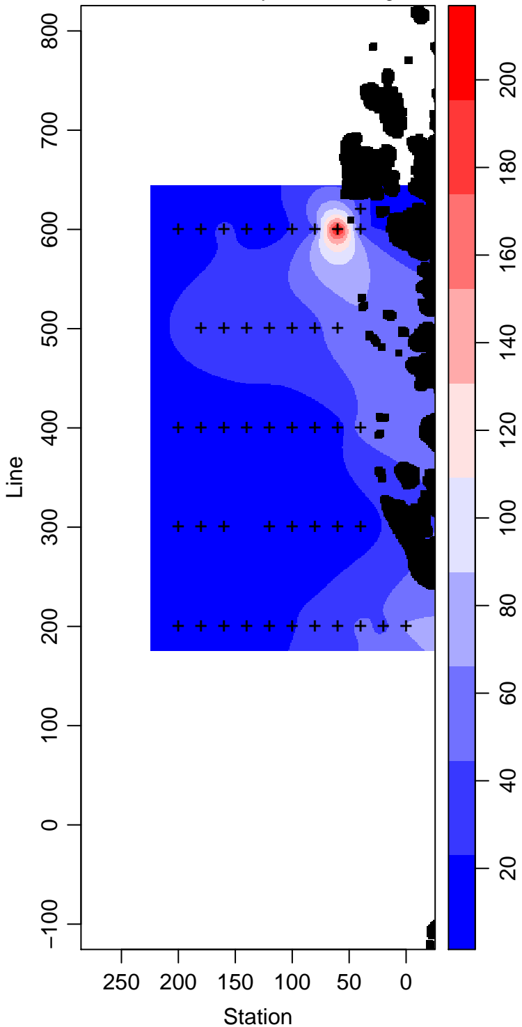
PD95-01_10_Primary.Production mg m -3
