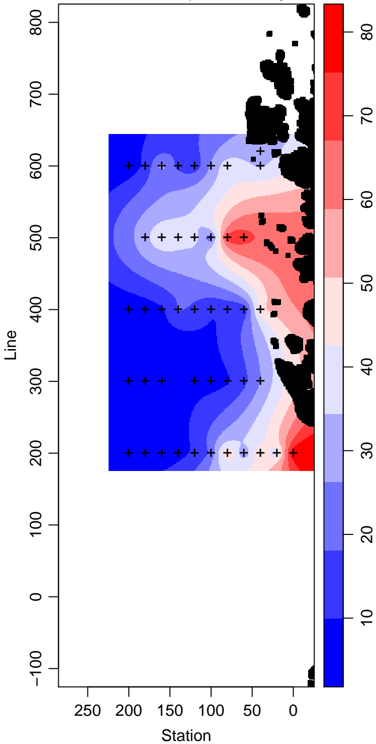
PD95-01_15_Primary.Production mg m -3
