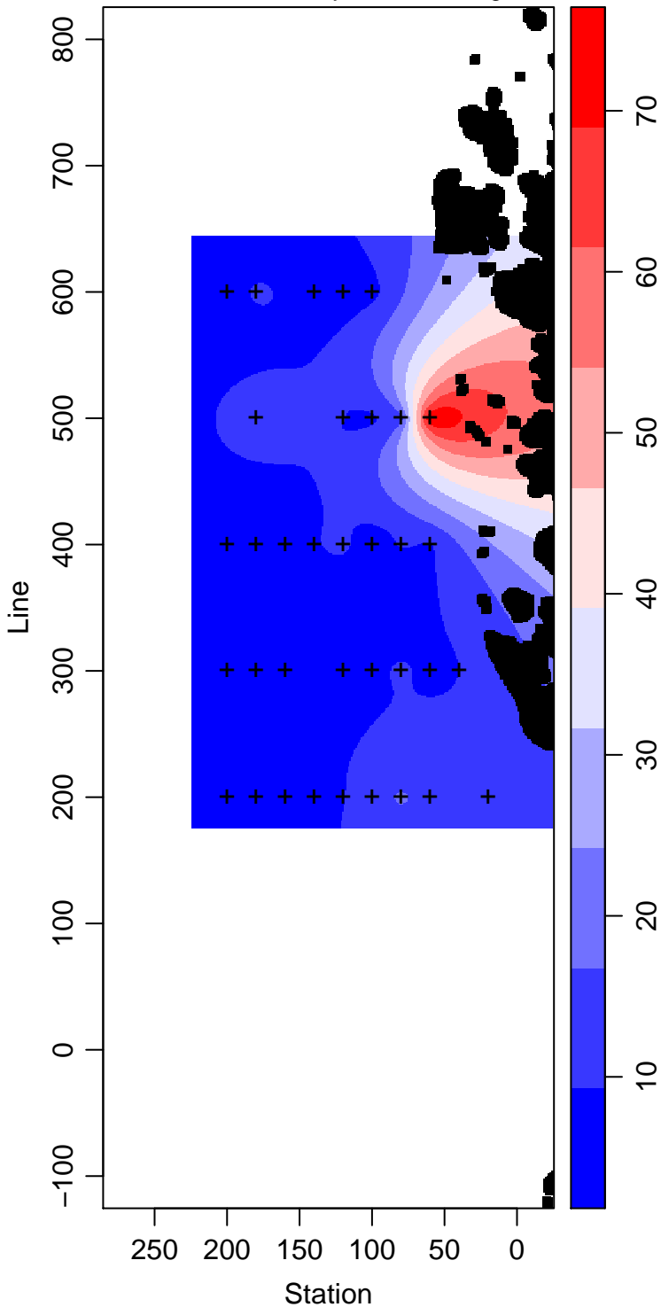
PD95-01_40_Primary.Production mg m -3
