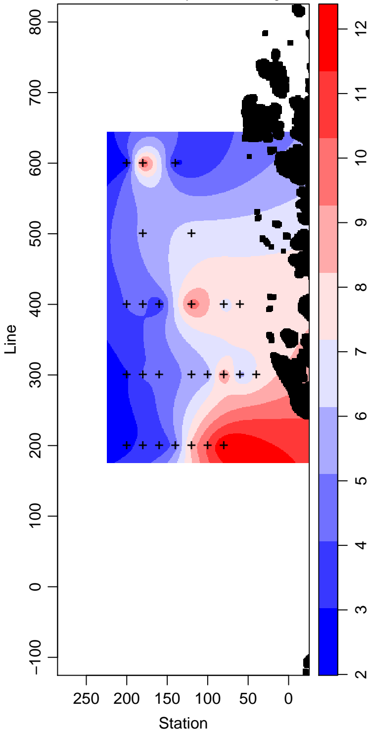
PD95-01_45_Primary.Production mg m -3
