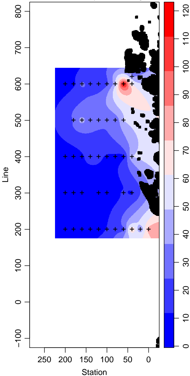
PD95-01_5_Primary.Production mg m -3
