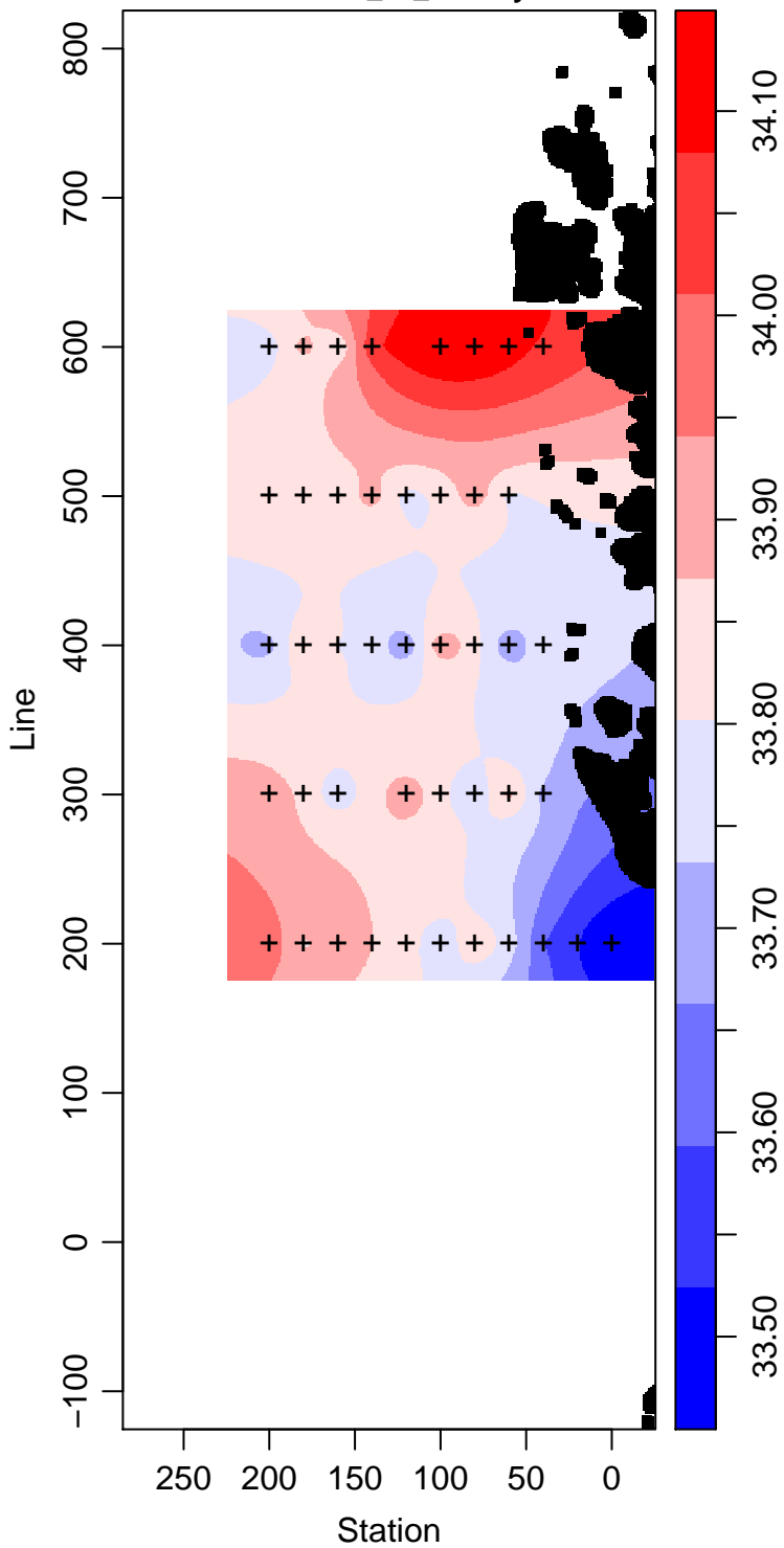
PD95-01_70_Salinity
