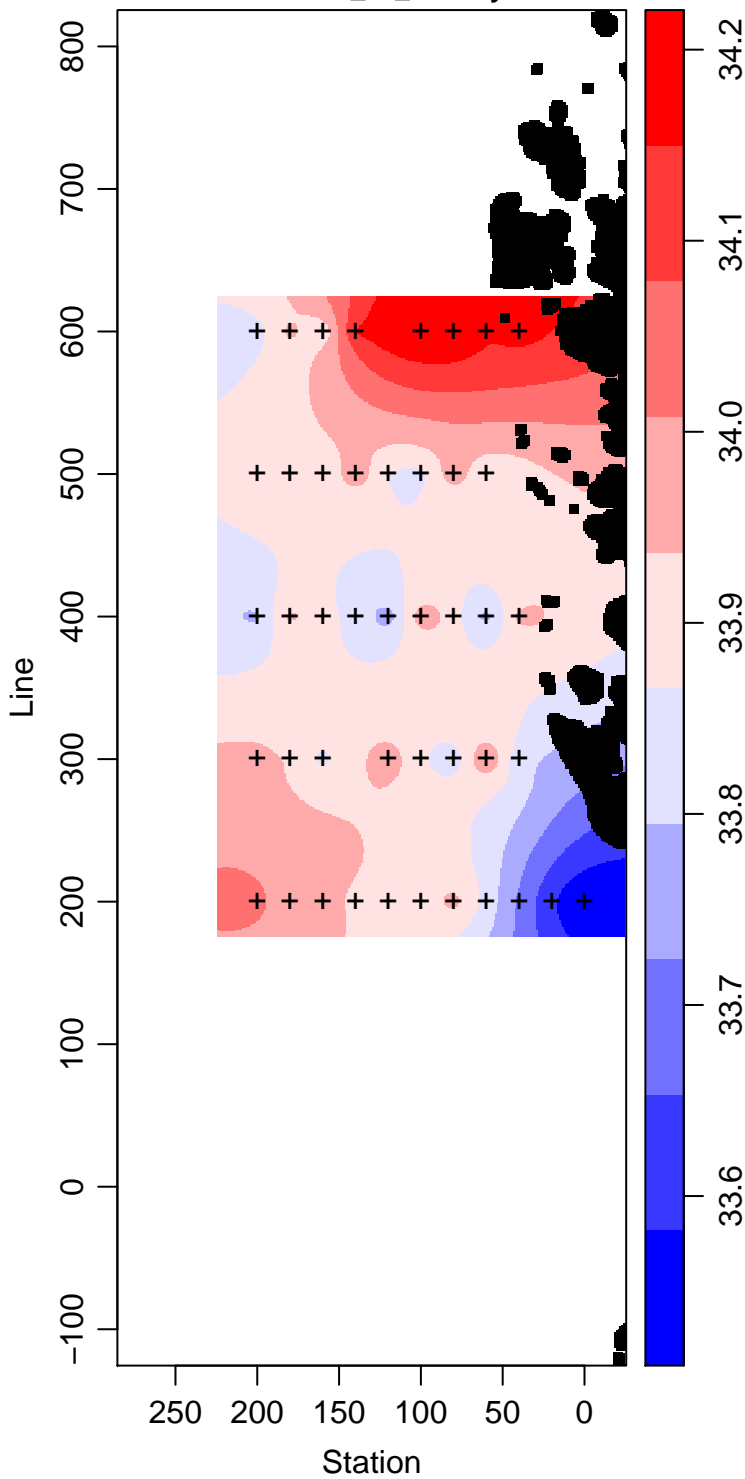
PD95-01_80_Salinity
