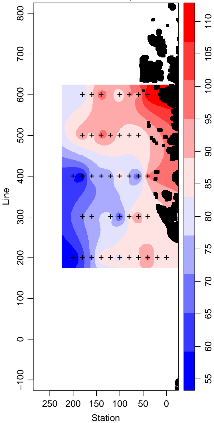
PD95-01_100_Silicate \mu\text{ mol L}^{-1}
