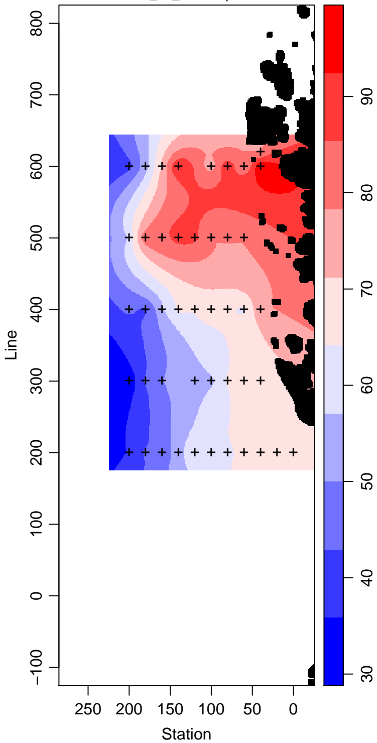
PD95-01_20_Silicate \mu\text{ mol L}^{-1}
