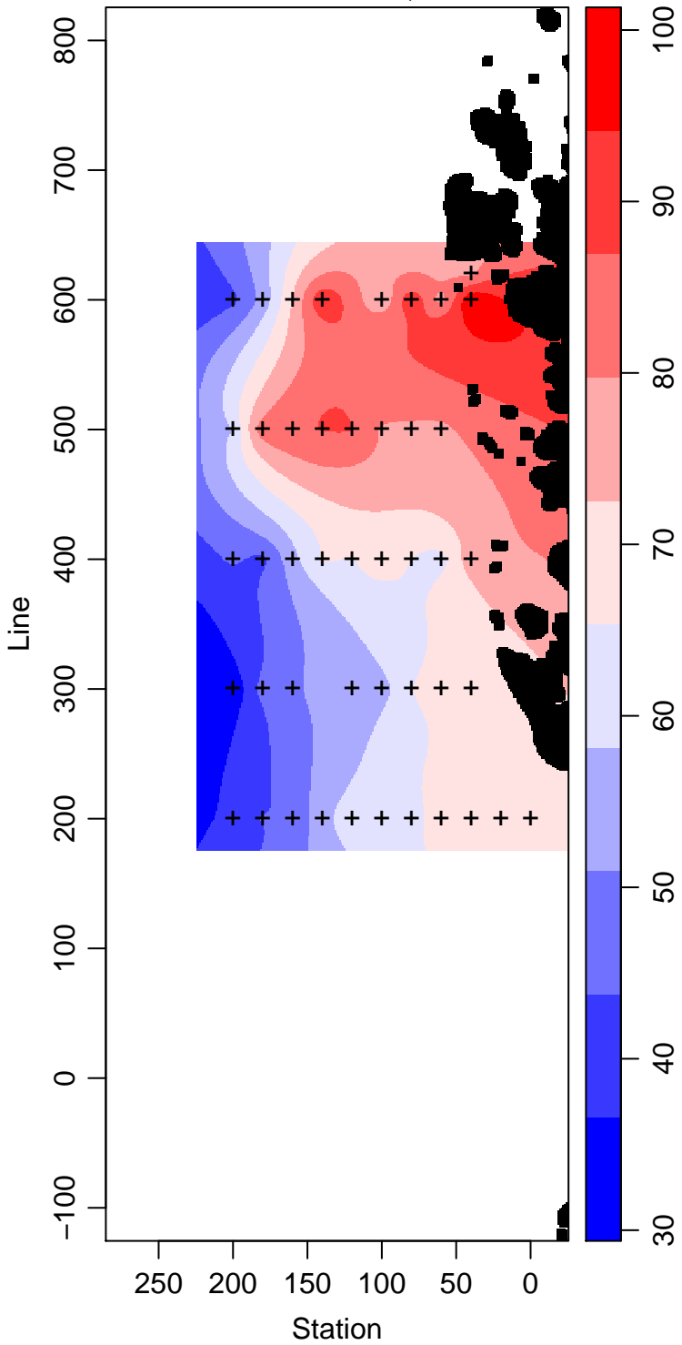
PD95-01_25_Silicate \mu\text{ mol L}^{-1}
