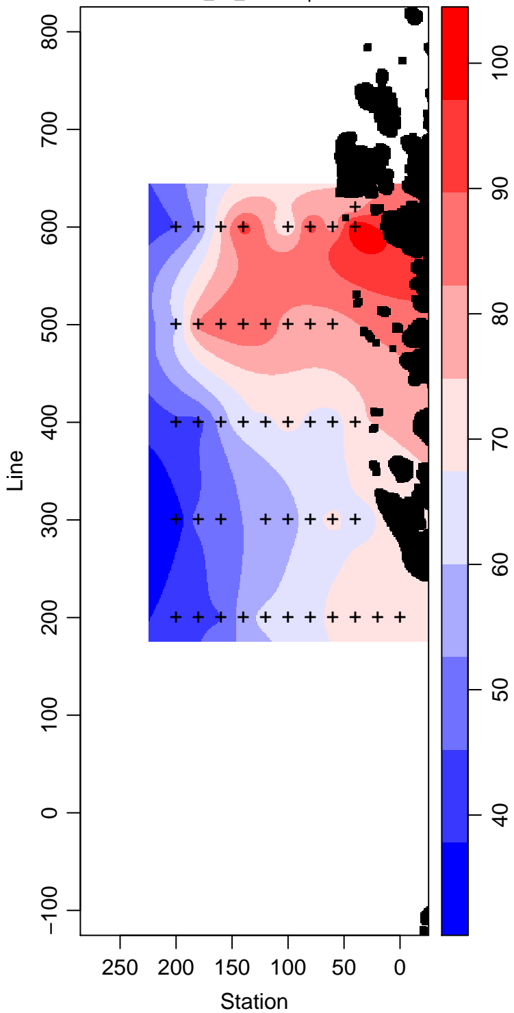
PD95-01_30_Silicate \mu\text{ mol L}^{-1}
