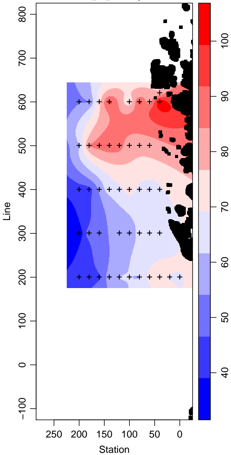
PD95-01_35_Silicate \mu\text{ mol L}^{-1}
