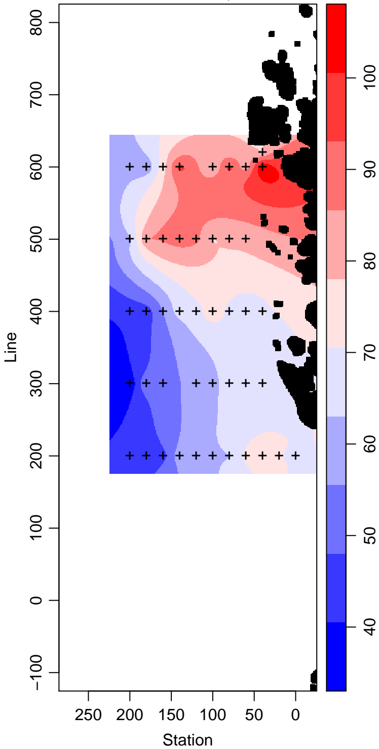
PD95-01_40_Silicate \mu\text{ mol L}^{-1}
