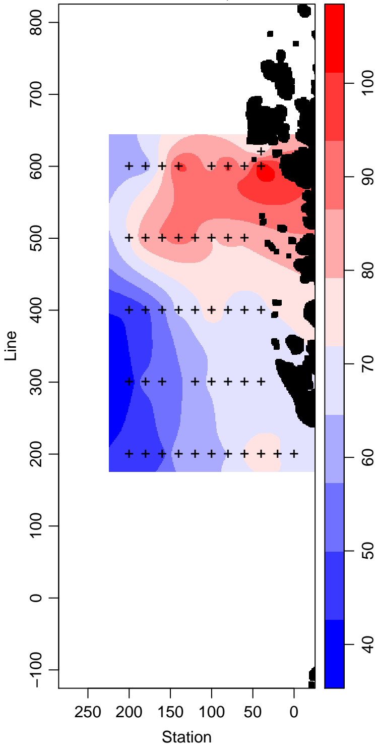
PD95-01_45_Silicate \mu\text{ mol L}^{-1}
