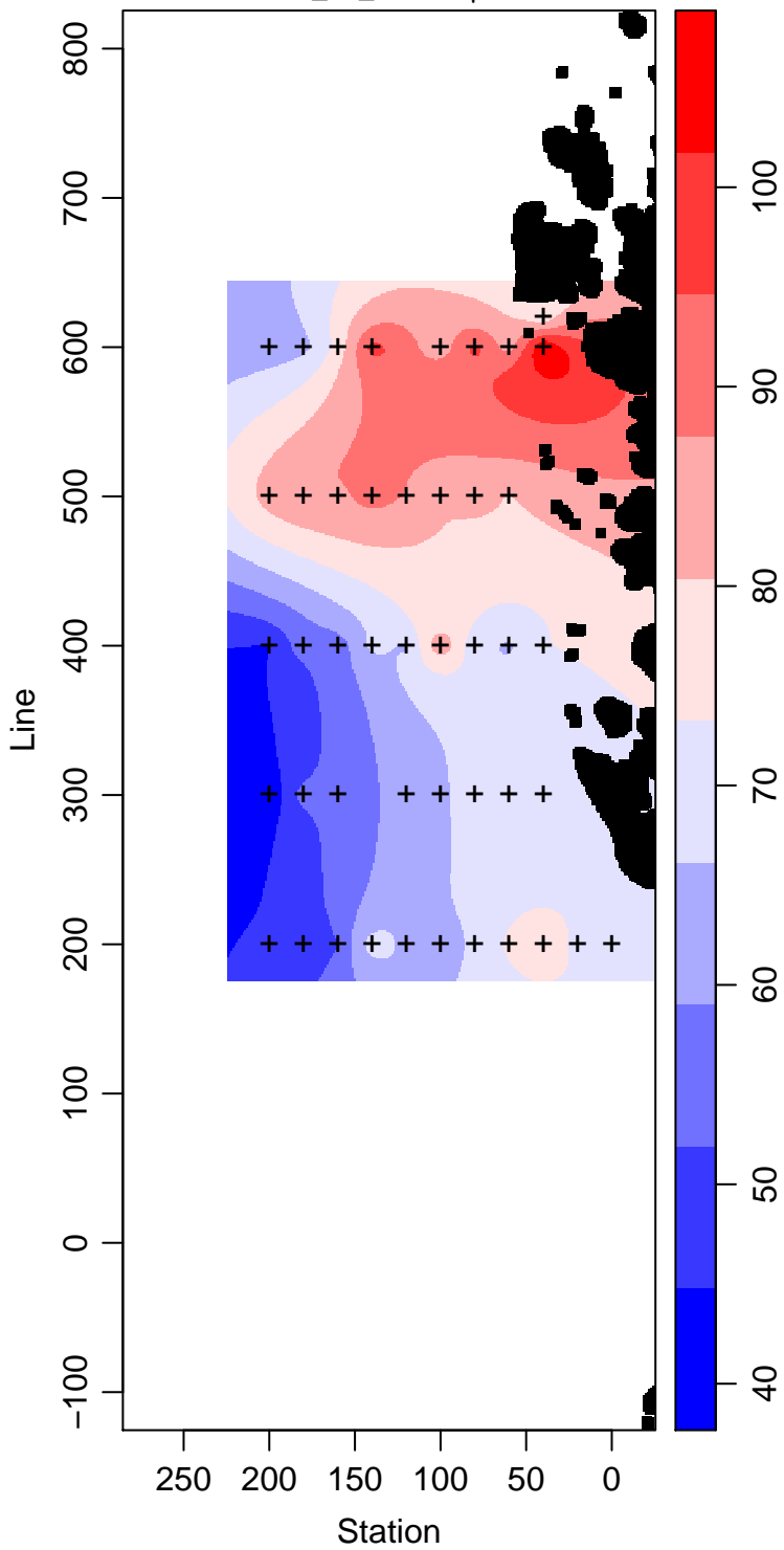
PD95-01_50_Silicate \mu\text{ mol L}^{-1}
