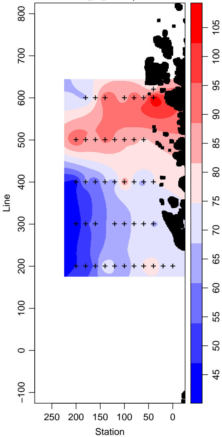
PD95-01_55_Silicate \mu\text{ mol L}^{-1}
