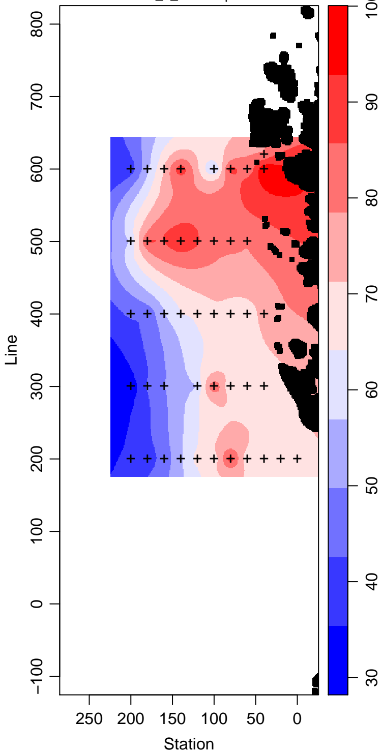
PD95-01_5_Silicate \mu\text{ mol L}^{-1}
