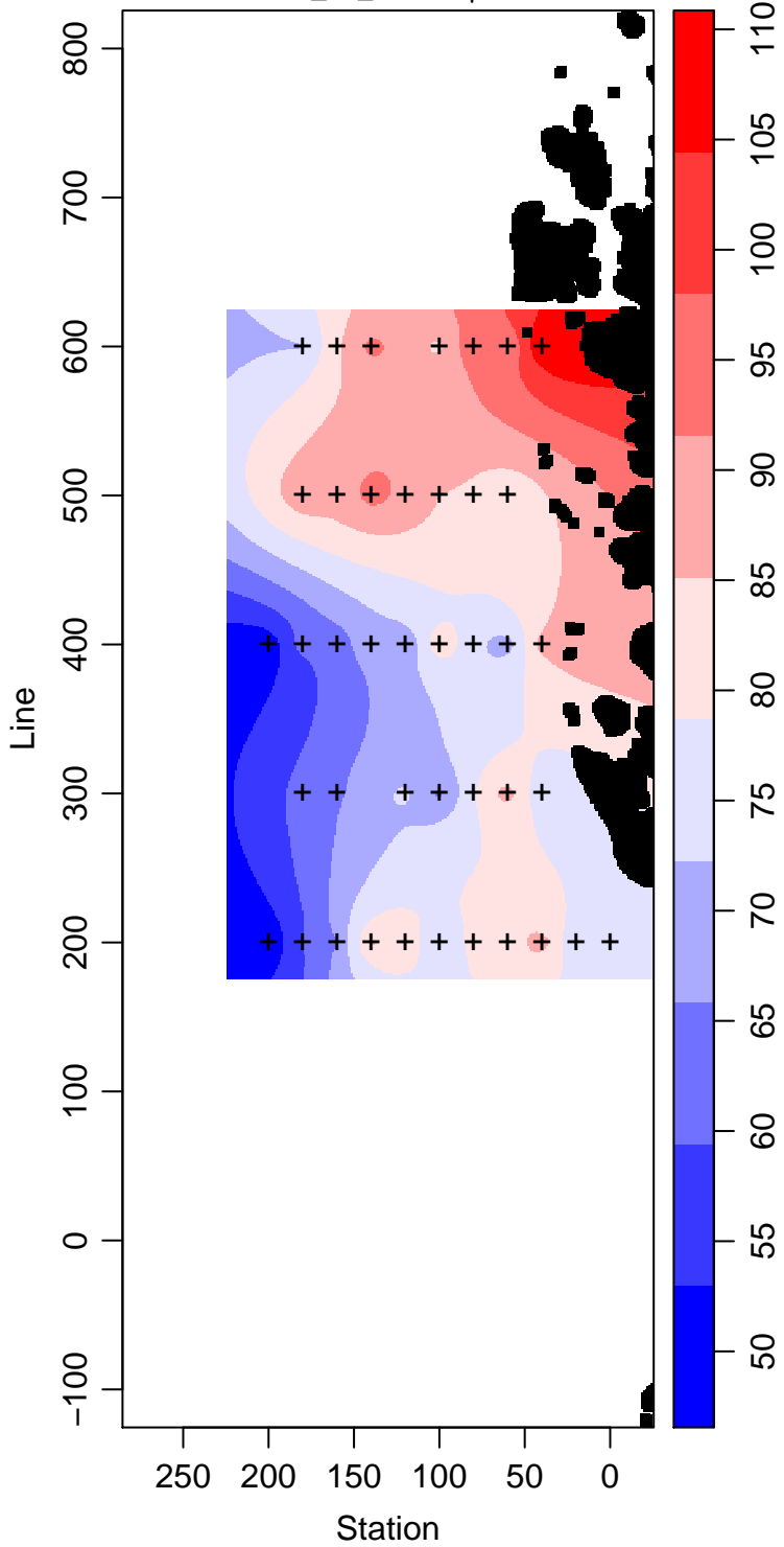
PD95-01_75_Silicate \mu\text{ mol L}^{-1}
