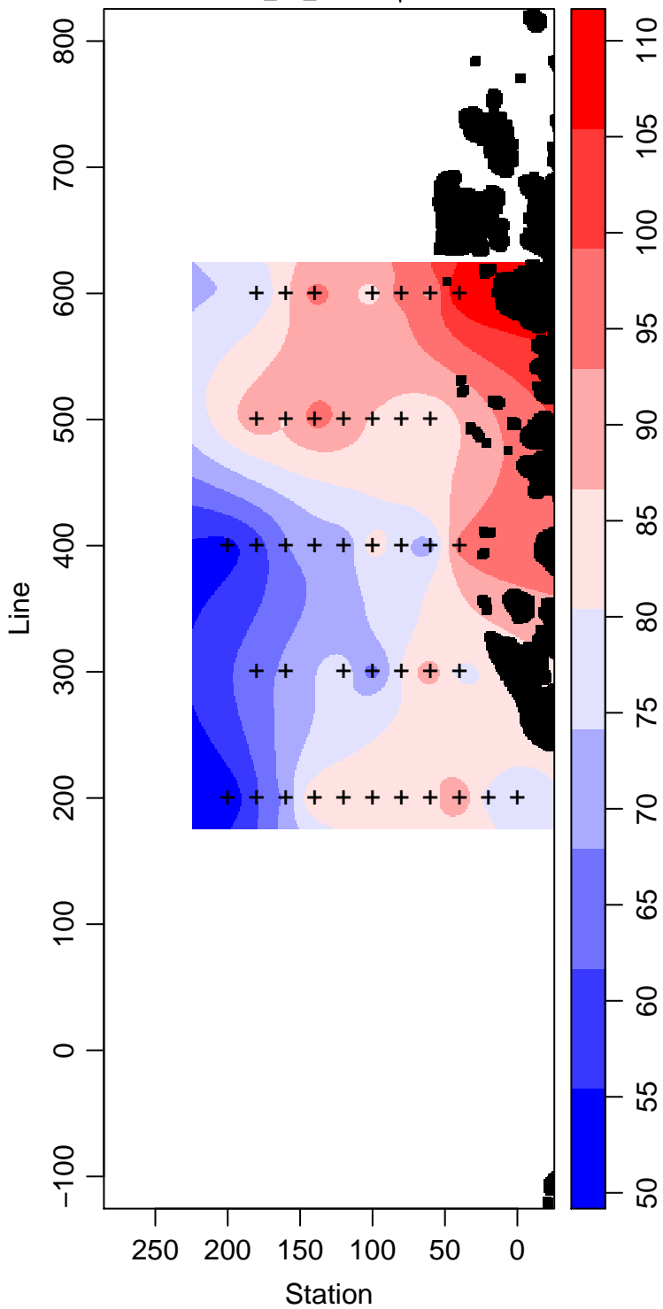
PD95-01_85_Silicate \mu\text{ mol L}^{-1}
